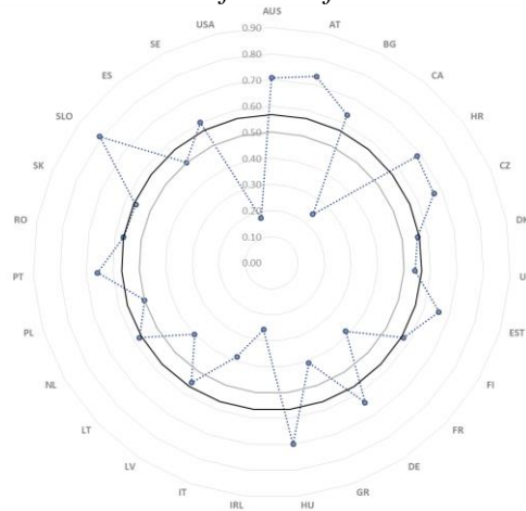
Figure 1. Comparison of the BLSI measure values for the analysed countries and against the median and middle value of BLSI of 0.5
